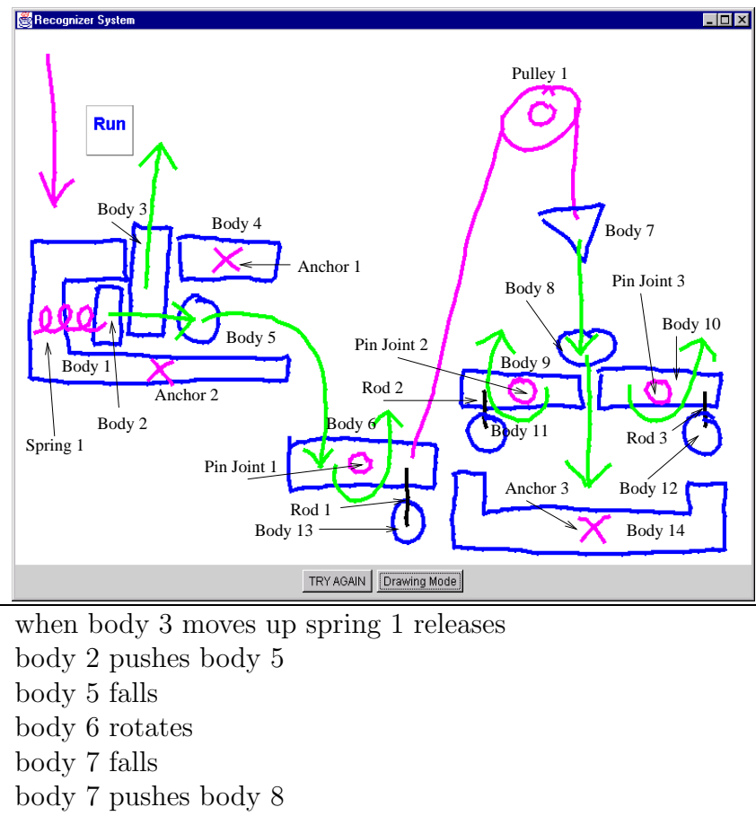
Figure 3-1: The description of the egg-cracker: The arrows in the sketch are gestures made by the designer and they describe the motions of the bodies. Below the sketch is a transcript of the utterances that made up the verbal part of the explanation.
